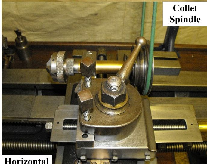
Horizontal Cutting Frame
