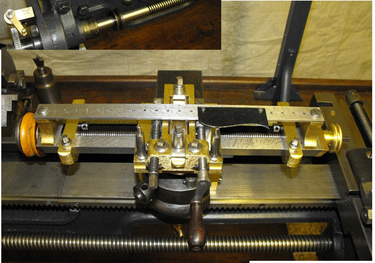
Ornamental Slide-rest with Fluting Stops and Curvilinear Apparatus
